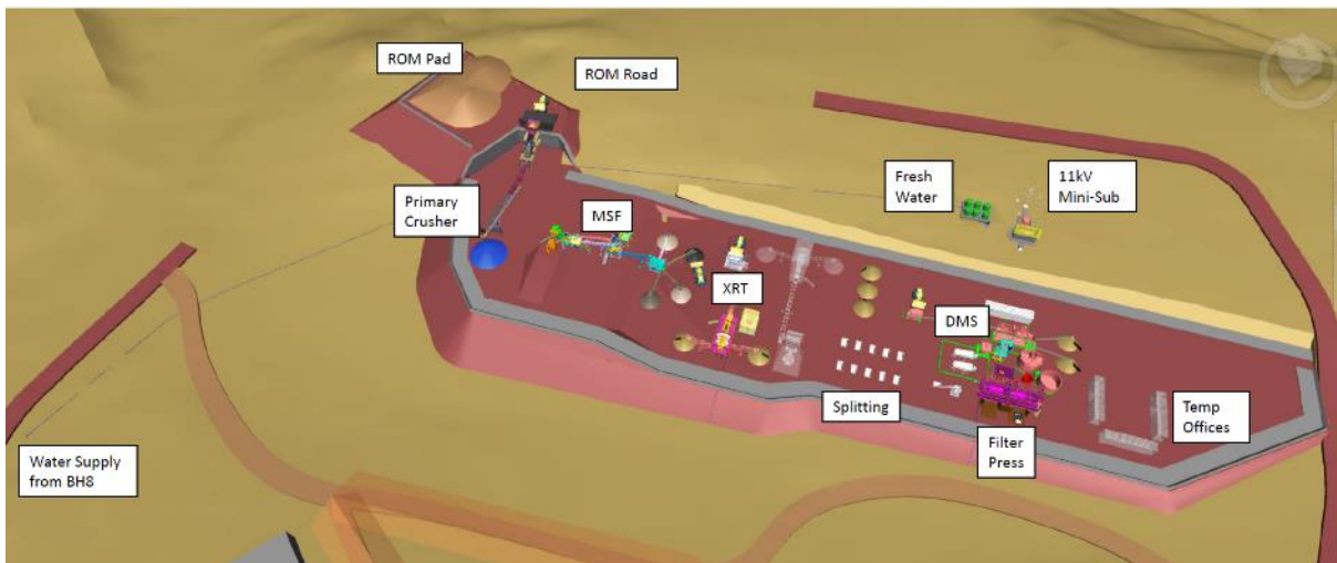
Figure 2: Three-dimensional model of the lithium pilot plant.
