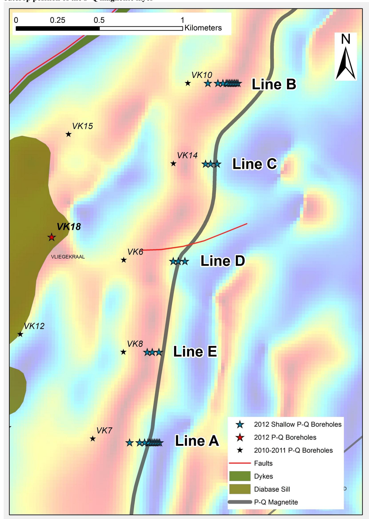
Figure 3: Localities of shallow boreholes drilled into the weathered zone and shown in relation to the outcrop position of the P-Q magnetite layer
