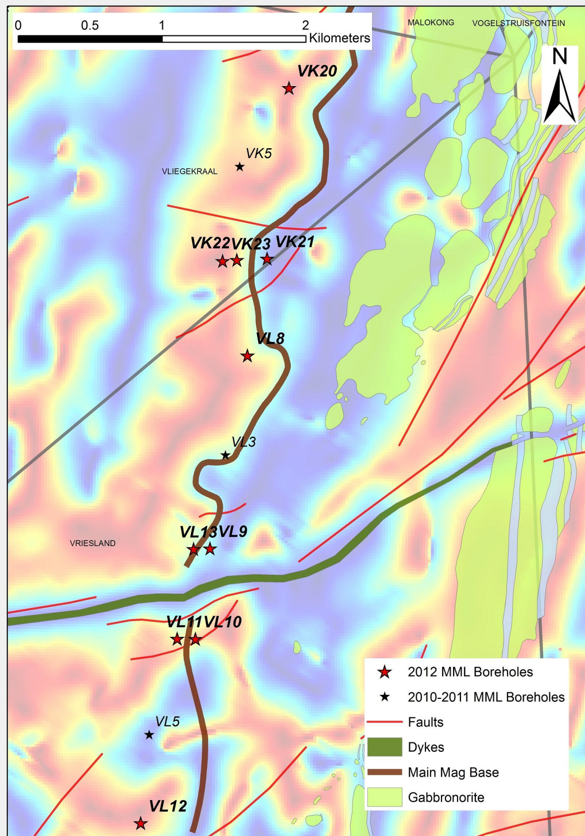
Figure 2: Borehole localities in relation to the outcrop position of the main magnetite layer shown with respect to the airborne magnetics and the position of dykes and sills
