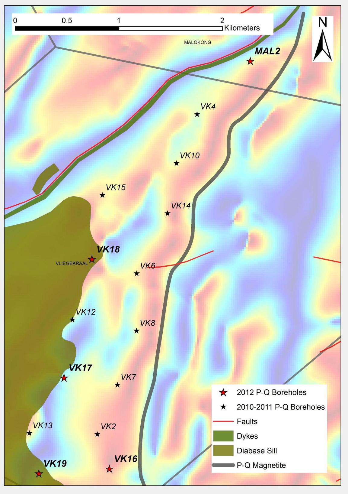
Figure 1: Borehole localities in relation to the outcrop position of the P-Q magnetite layer and shown with respect to the airborne magnetics and the position of dykes, sills and faults
