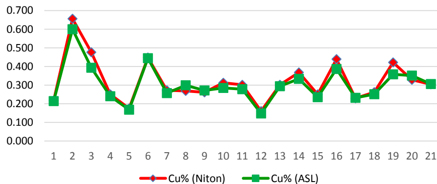
Niton Vs. Alex Stewart Laboratory Analyses Copper Comparison
