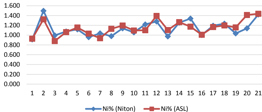
Niton Vs. Alex Stewart Laboratory Analyses Nickel Comparison
