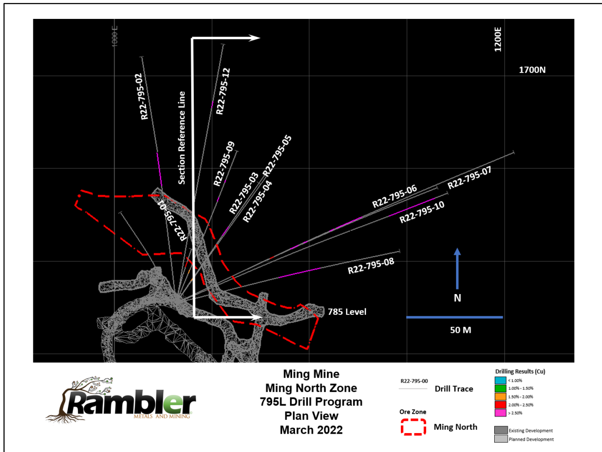
Figure 5: Plan view of 795L drill program
