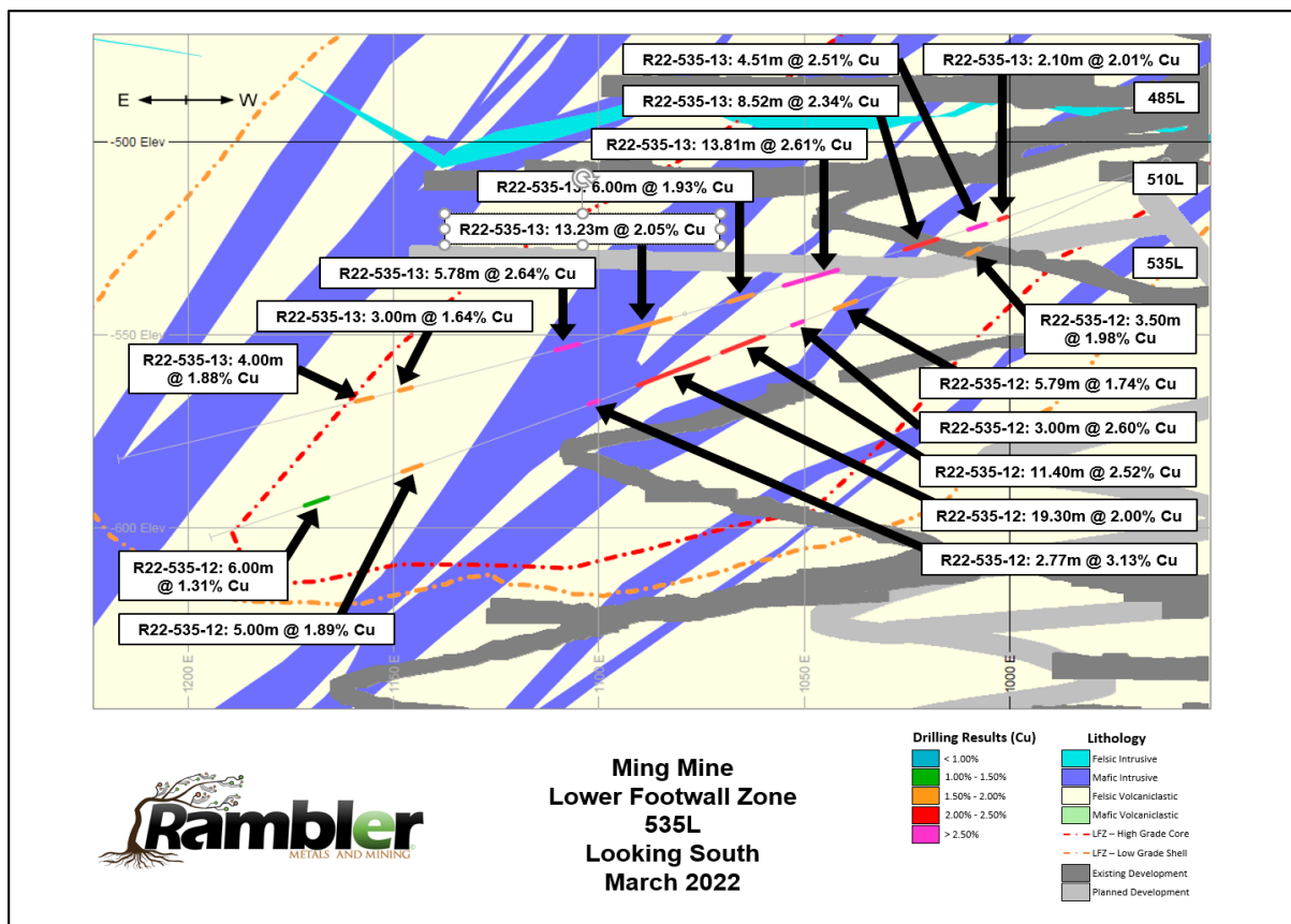
Figure 4: Section view of 535L holes 13 and 14, looking south
