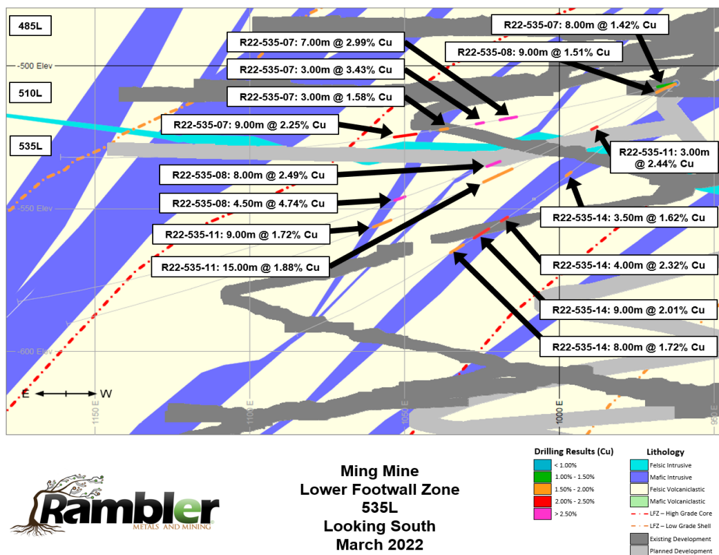
Figure 2: Section view of 535L holes 7, 8, 11, and 14, looking south
