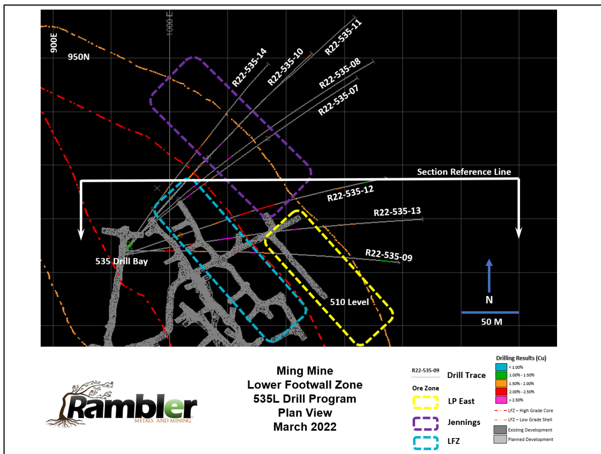
Figure 1: Plan view of 535L drill program
