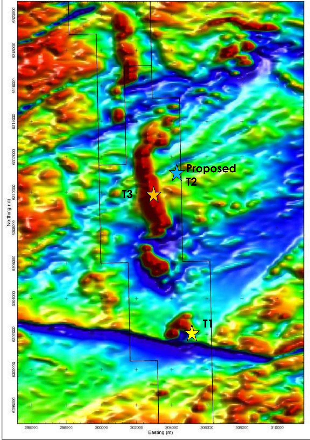
Regional TMI Magnetic Image - Survey Area 4
