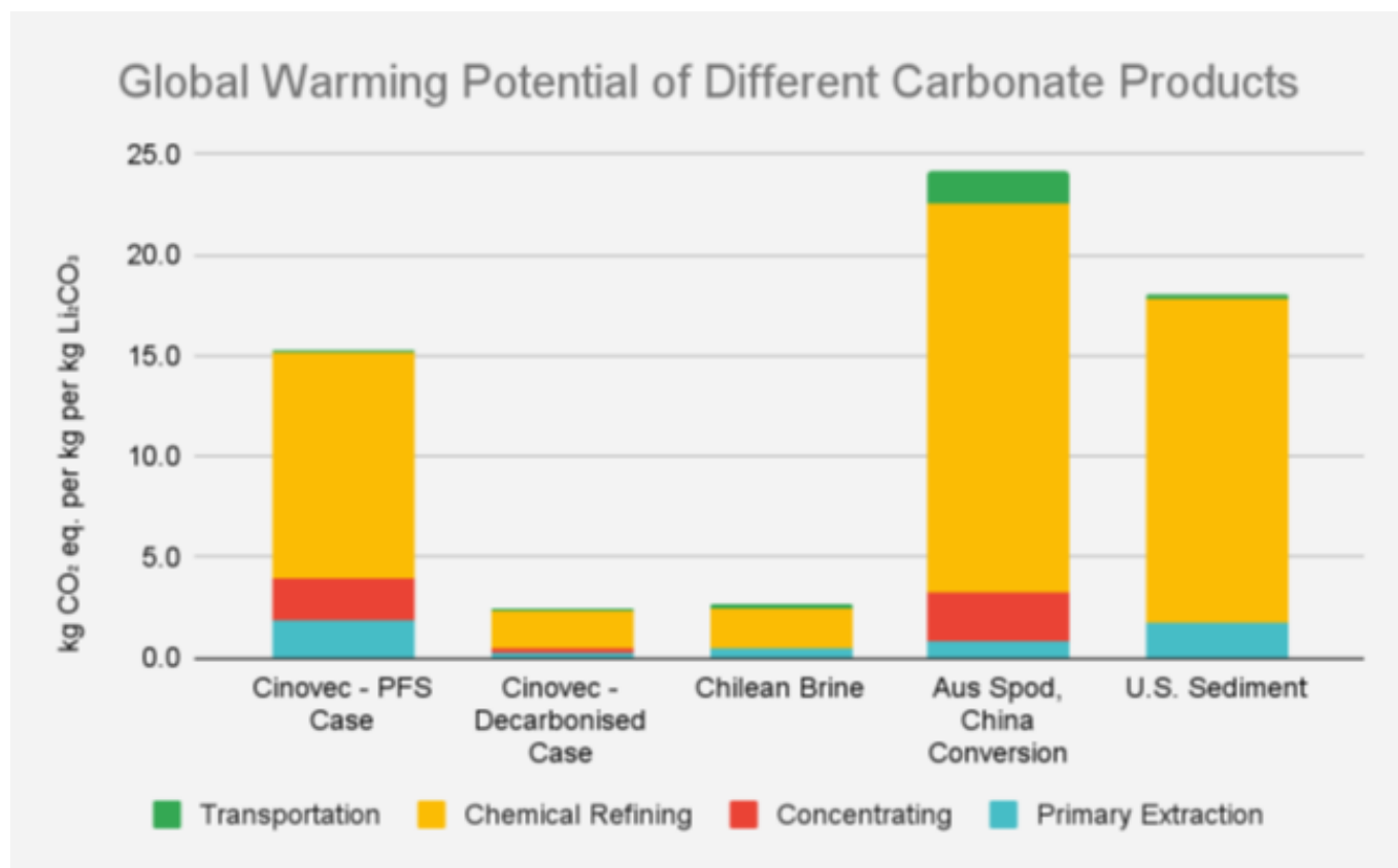
Figure 2: GWP Impact of \text{Li}_2\text{CO}_3 produced from Cinovec PFS (2019), the theoretical Cinovec Decarbonised Case, for Chilean Brine, Australian Spodumene converted in China, and US Sedimentary Clay. Source: Minviro
