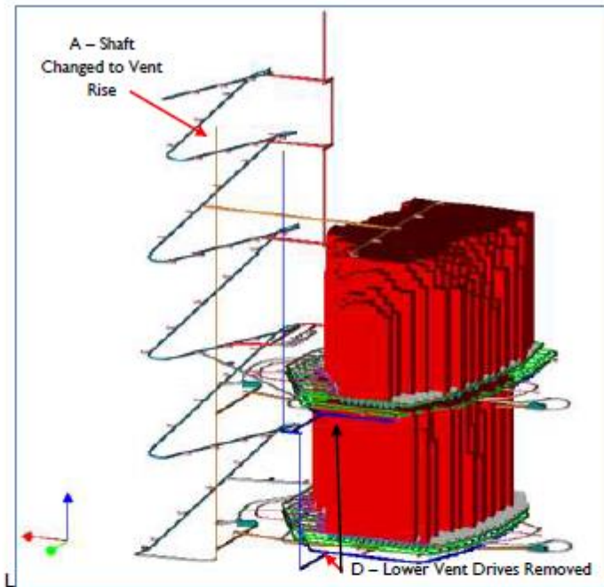
Figure 1: Guinaoang Copper Project - original 2011 scoping study mine design
