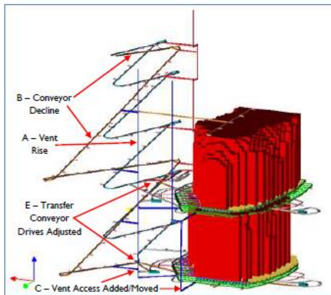
Figure 2: Guinaoang Copper Project - adjusted mine design
