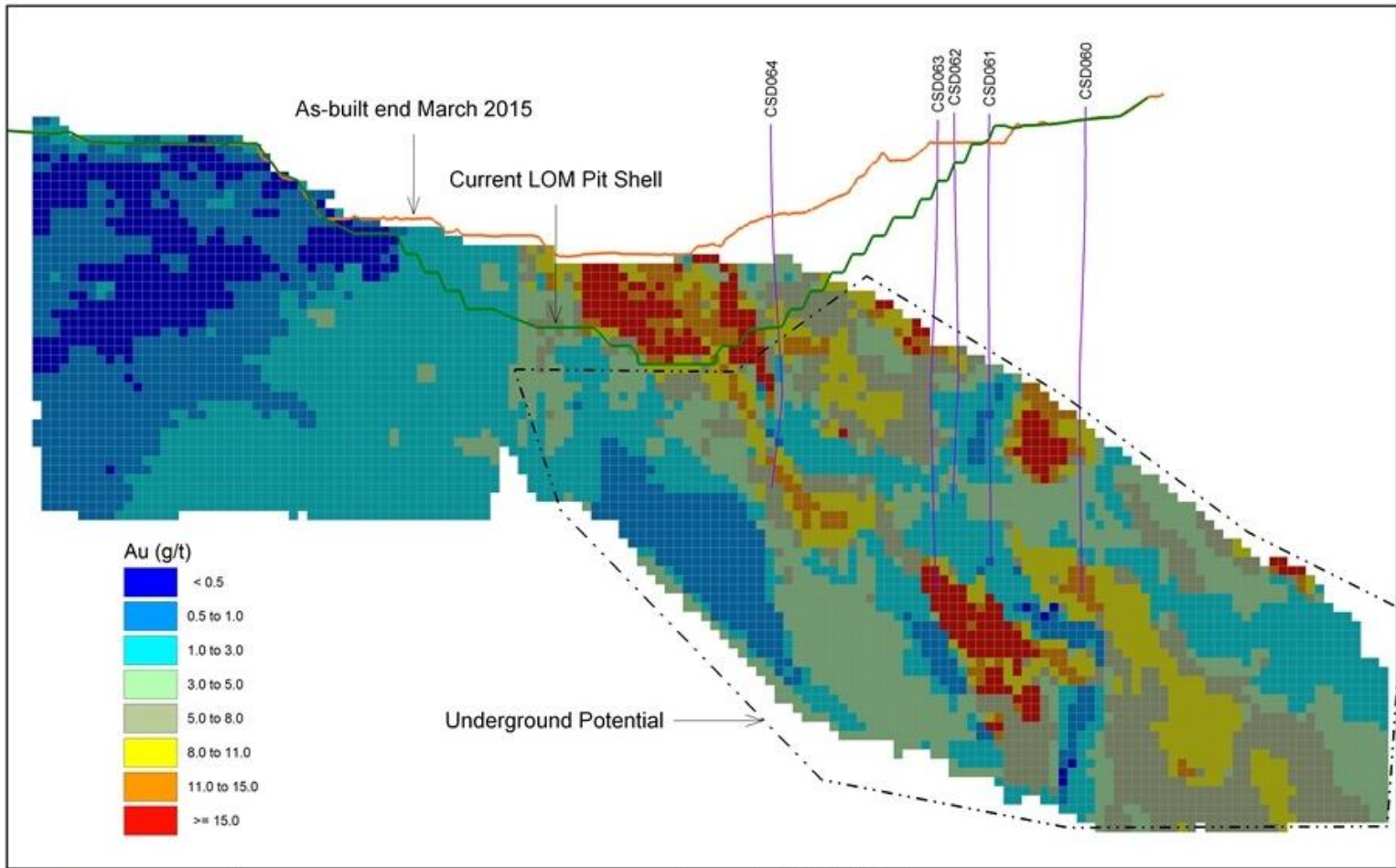
Figure 1: Bauhinia Creek Deposit April 2015. Long Section Looking South Depicting Resource Model, Recent Drill Hole Traces and open pit Outline
