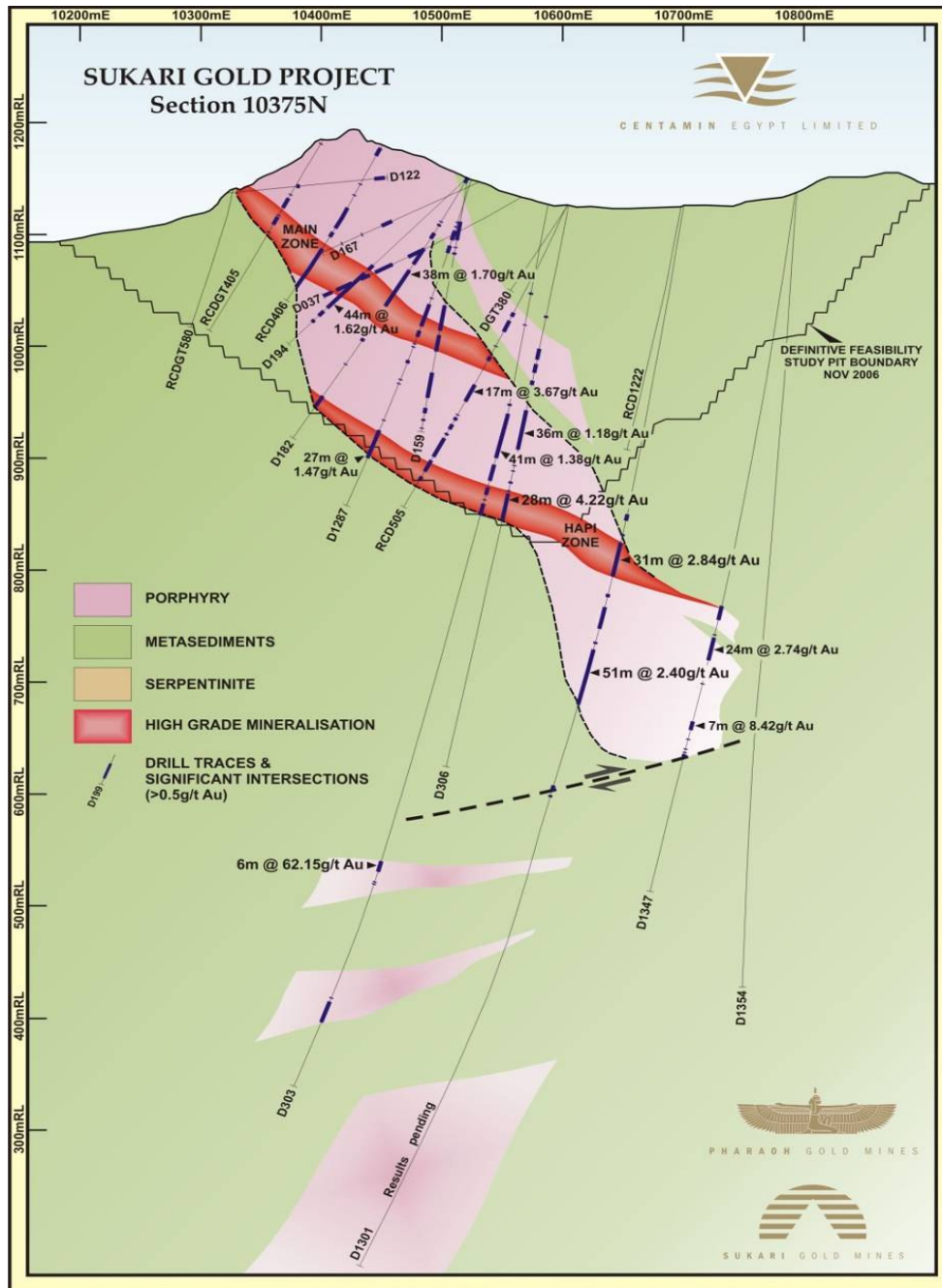
Figure 4 – 10375N showing high grade intersection in D303 in the downthrust zone and thick mineralised porphyry block of the Horus Zone in D1301 (results awaited)
