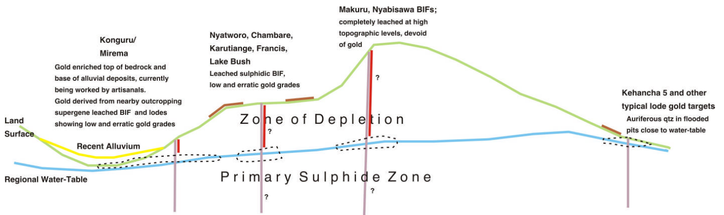
Schematic of Supergene Effects on Gold Grades in Sulphidic Mineralisation and Reworked BIFs, Migori Belt, Kenya
