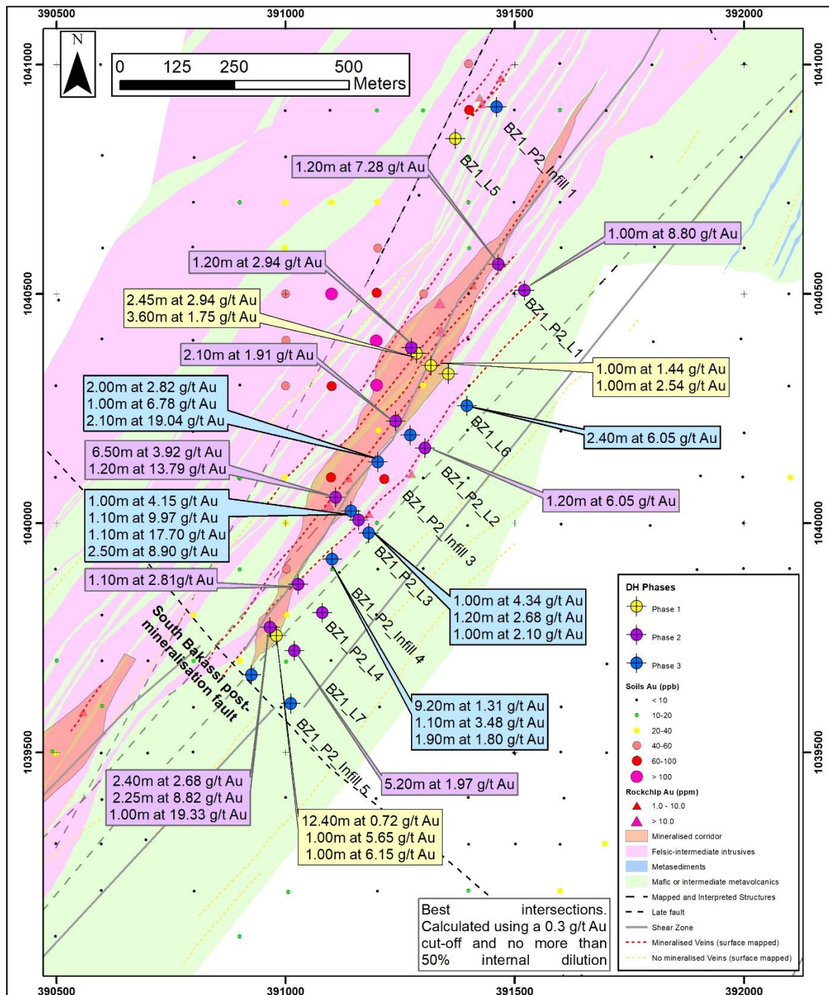
Diamond Drill Plan Summarising Best Intersections to Date at Bakassi Zone 1. Results for Phase 3 are Shown in Blue
