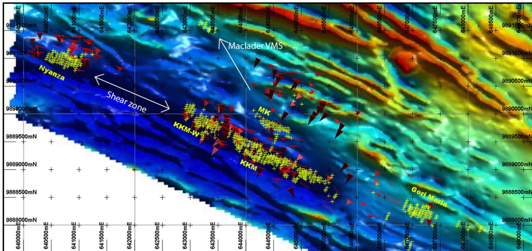
Figure 1: Total field aeromagnetic imagery for the Migori area collected by Red Rock, with drill collars annotated in yellow and surface structural dip and dip-directions as red triangles
