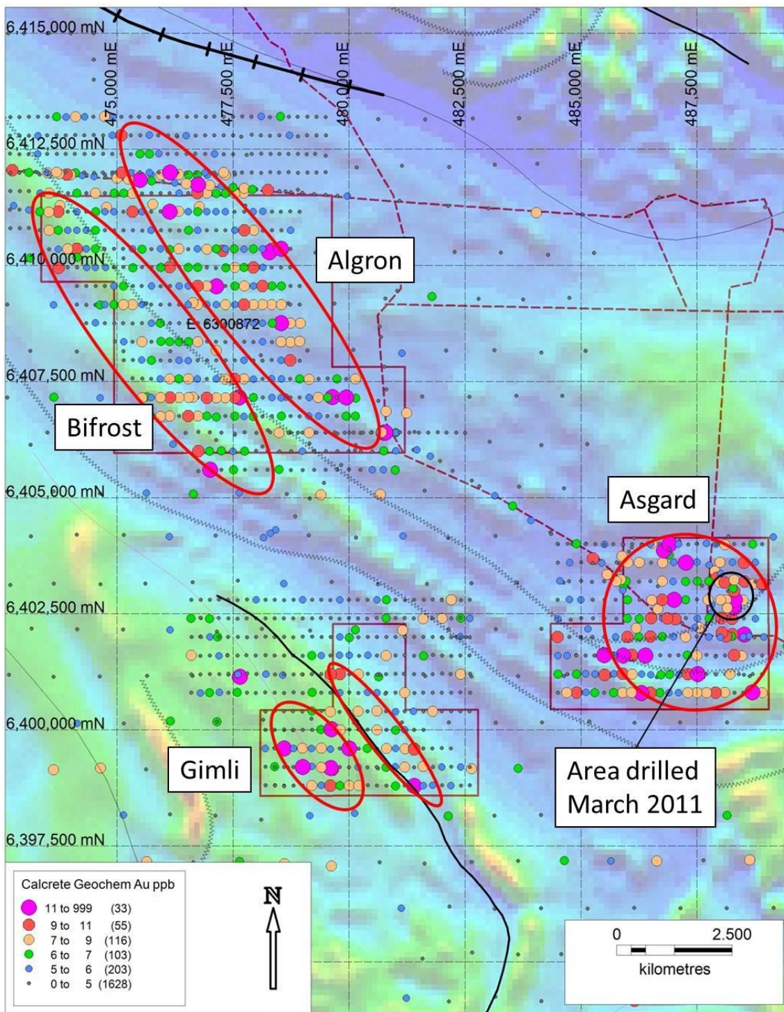
Figure 2: Calcrete Geochemistry Results
