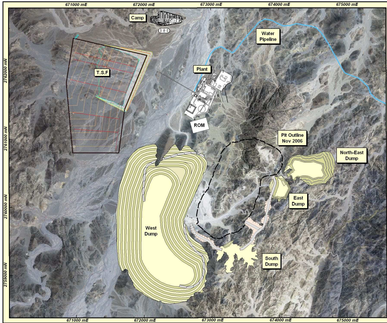
Figure 3: Sukari Project – Proposed Layout
