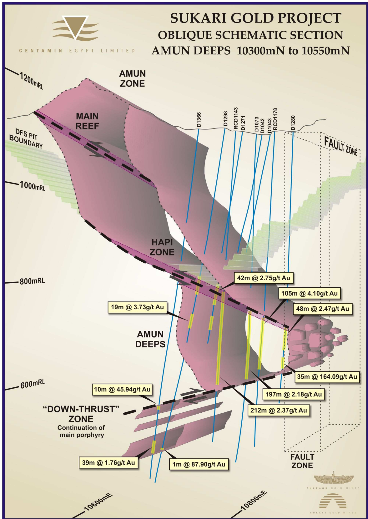
Figure 6 - Schematic Cross Section across the Amun Deeps Zone, showing main structural features, some drilling and assay intersections
