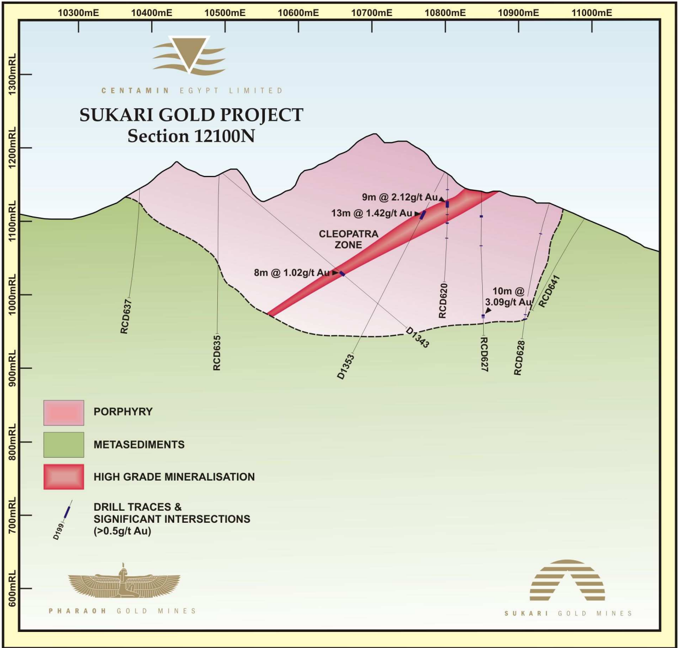
Figure 14 – Schematic Section 12100N – West Dipping Cleopatra Zone, far north Pharaoh Zone
