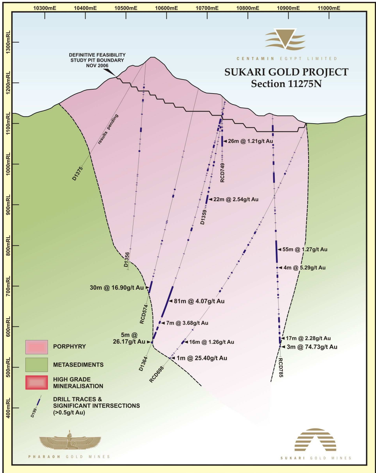
Figure 13 – Geological Section 11275N – Pharaoh Zone; high grade up-dip Hapi Zone in D1364, footwall geometry
