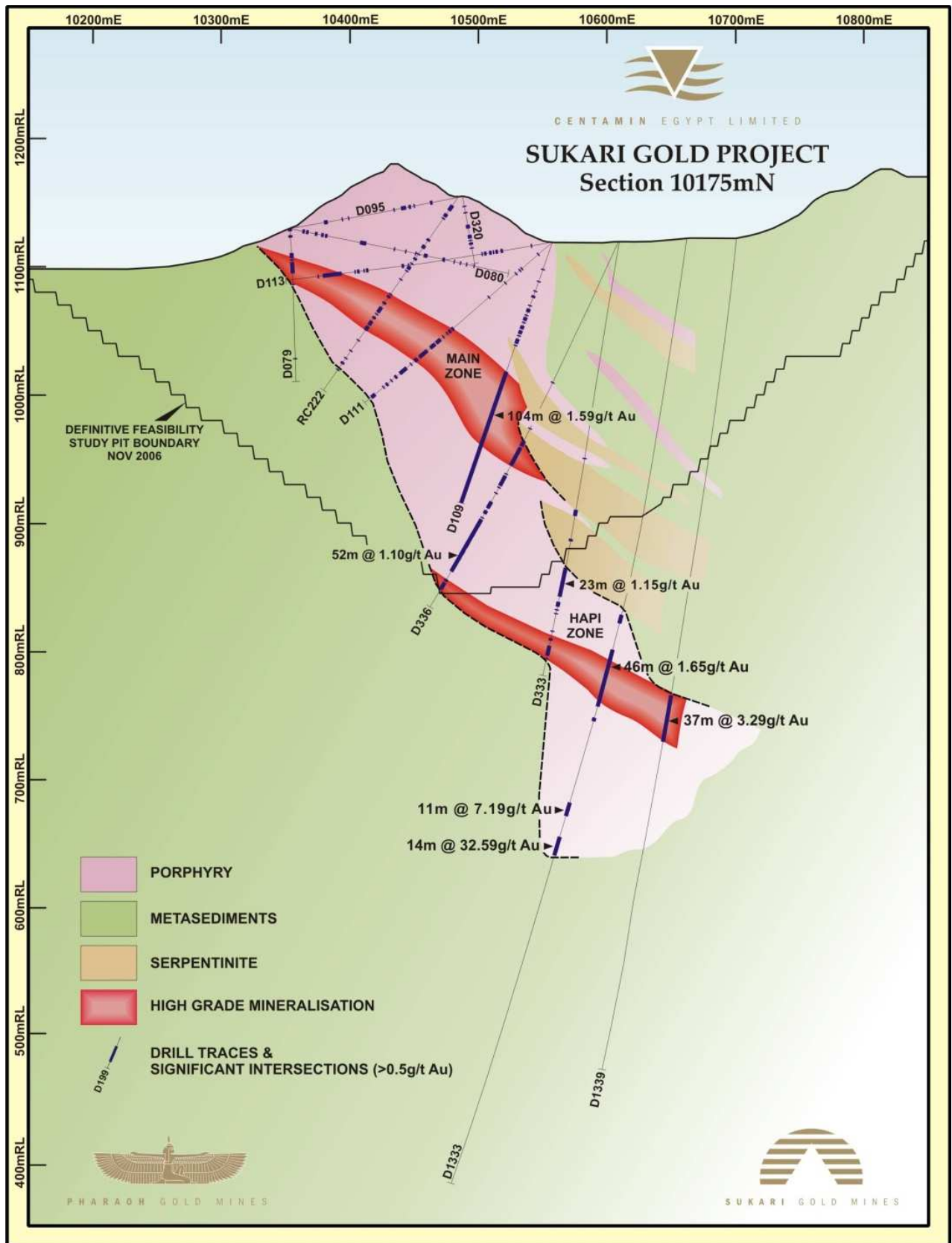
Figure 11 – Schematic Geological Section 10175N – Holes D1333 and D1339
