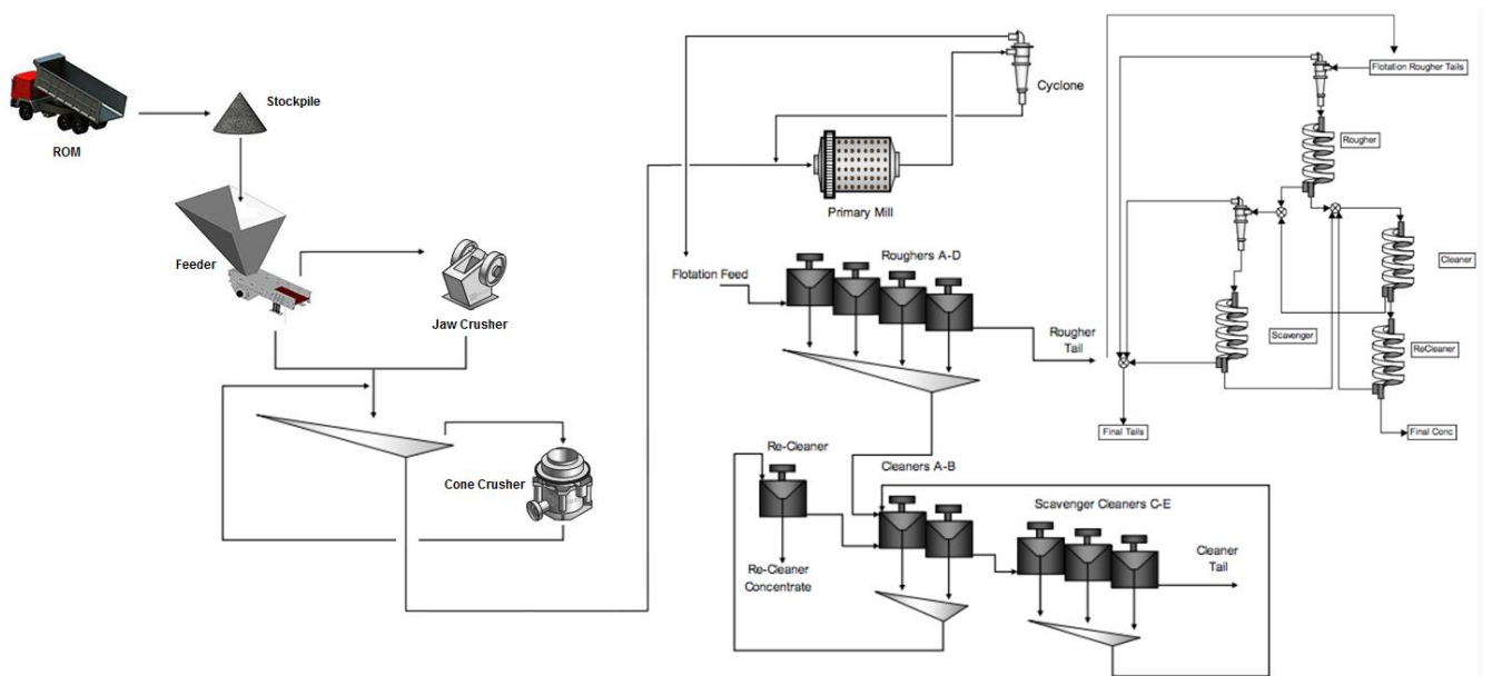
Figure 2: Conceptual flowsheet for the Pedra Branca PGM project
