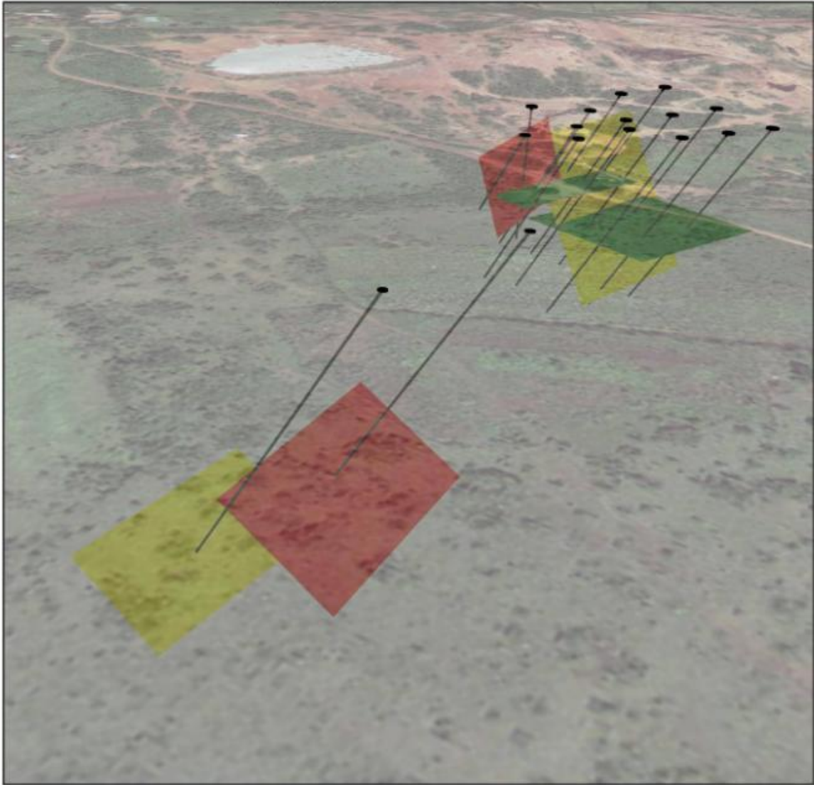
3D Plate Models with Phase 1 RC drilling facing South West
