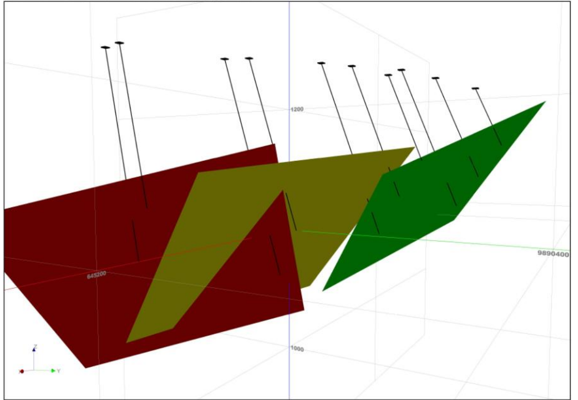
3D Partial Plate Models with Phases 1 and 2 RC drilling facing South West
