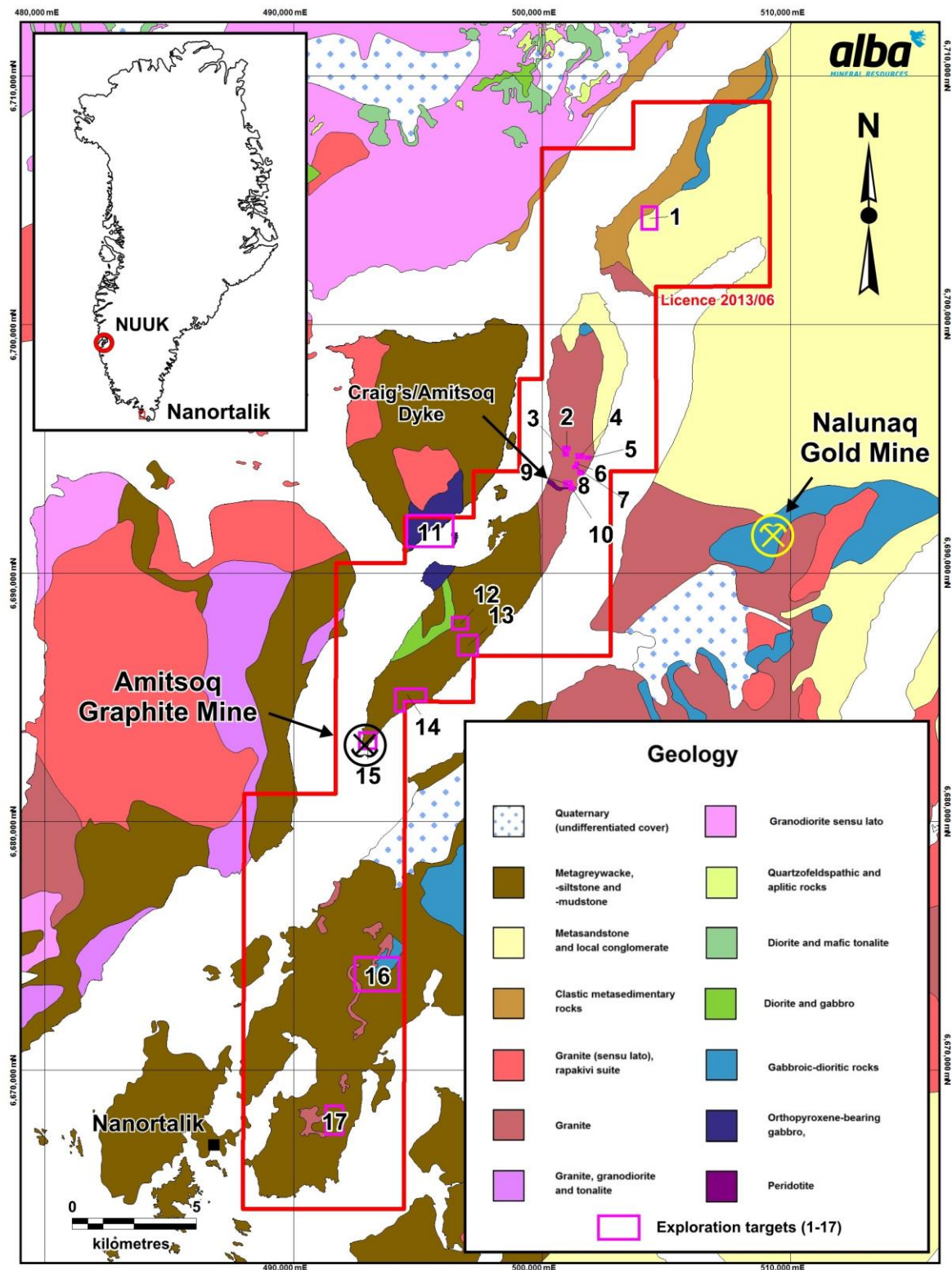
Figure 2. Location of the Amitsoq licence (2013/06) illustrating the underlying geology and targets (1-17) identified from the FeO remote sensing study.
